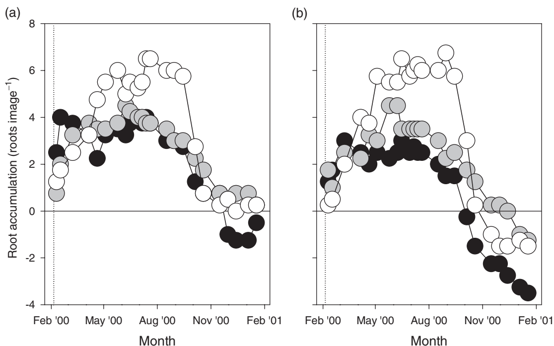
Fig. 3 Root accumulation at a depth of 4 cm during experiment 3, (a) in ambient temperature soil, (b) in warmed soil. Open symbols denote non-shaded, grey symbols 'half' shaded and black symbols 'full' shaded plots. Dotted lines represent start of treatments.
