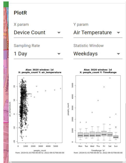
Fig. 5: Anomaly visualization with PlotR micro service.
