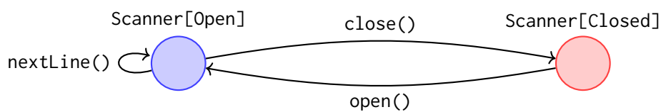
Figure 2.3: The Scanner typestate automata, based on Listing 1.3.
