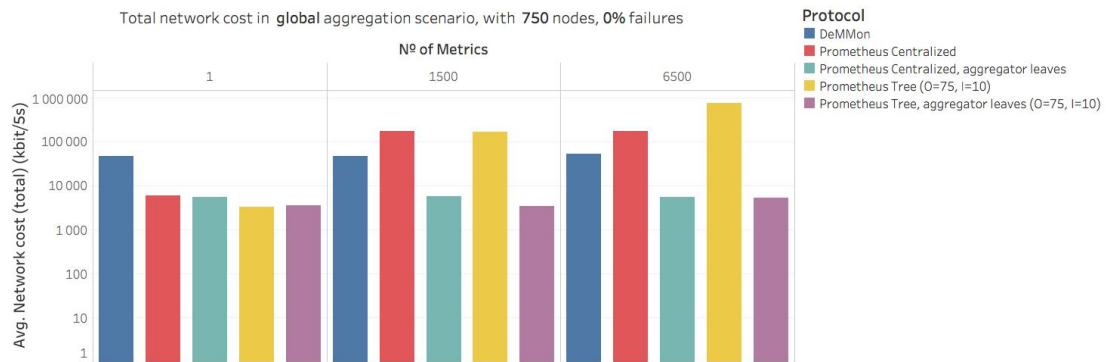
Figure 5.20: Average network cost incurred during global aggregation
