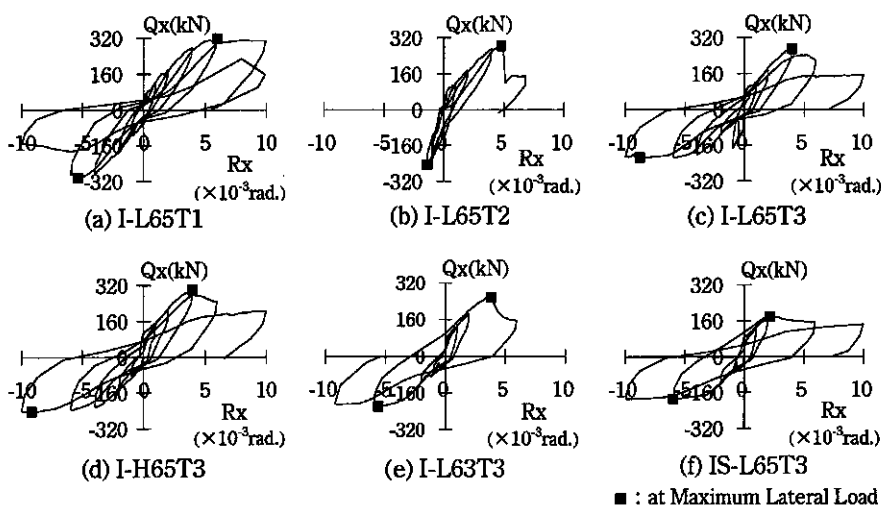
Fig. 7 Load-Deflection Curves
