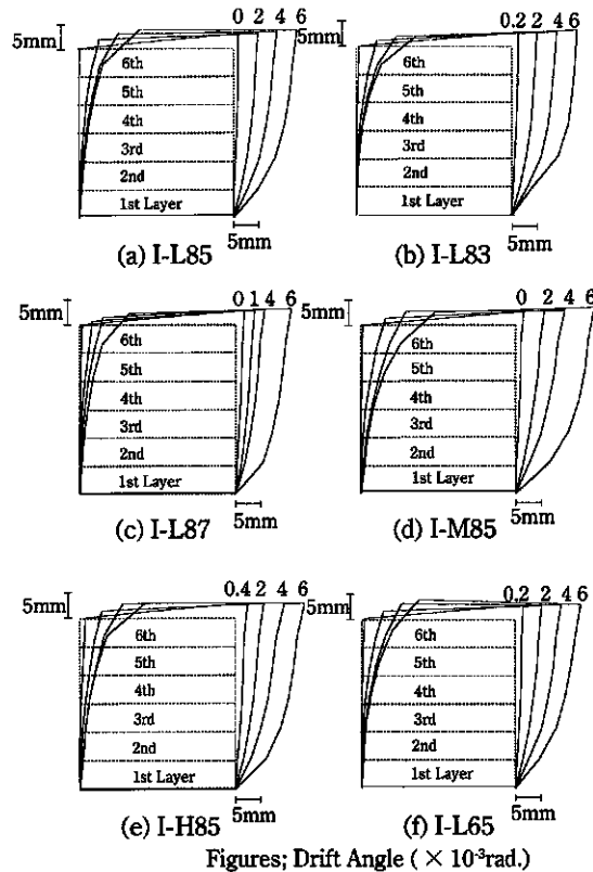
Fig. 8 Deformation Diagrams
