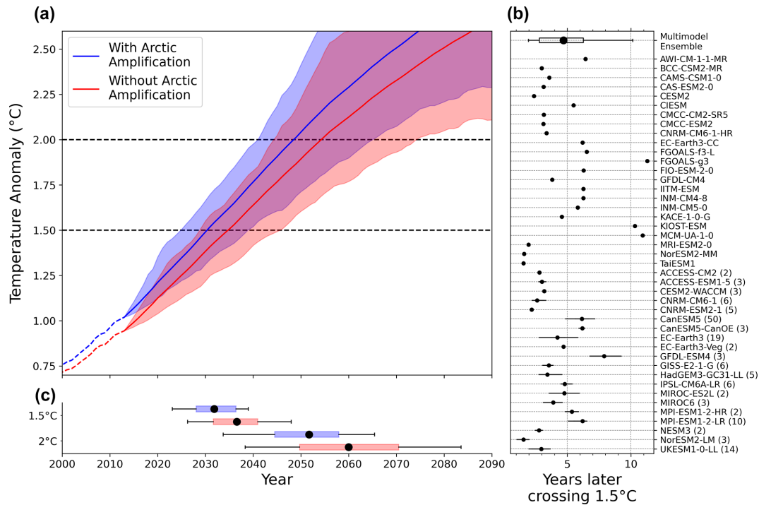
Figure 1. Effect of Arctic amplification on temperature rises above the Paris limits in CMIP6 models. (a) Observed and projected global mean temperature anomalies relative to the pre-industrial with and without Arctic amplification. The CMIP6 projections are constructed from the first ensemble member of each model’s SSP2-4.5 scenario, scaled to the observed present-day anomaly. All temperatures anomalies are 20-year, centred, rolling means. Central lines indicate multi-model means; shaded regions represent the spread between the 10 % and 90 % intervals. (b) Number of years later when each CMIP6 model breaches the 1.5 °C temperature threshold without Arctic amplification. Error bars show the range of this value across ensemble members, dots show the ensemble mean, and numbers in brackets following the model names indicate the number of ensemble members. For the multi-model ensemble, the box shows the 25th-to-75th percentile range, and whiskers show the 5th-to-95th percentile range. (c) Distributions of crossing years in the multi-model ensemble for the two temperature thresholds with and without Arctic amplification. The box plots are defined as in (b).
