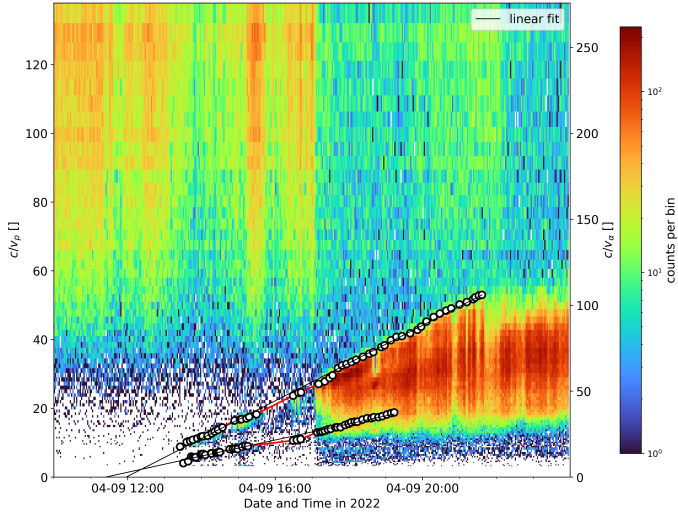
Fig. 5. EPT measurements from the magnet telescope plotted as inverse velocity (assuming that the particles are protons) vs. time. In this representation, ions that are released at the same time but have different velocities lie along a straight line. The upper curve shows “point-and-click” values for protons, the lower for helium nuclei as well as their linear fits. The left-hand y-axis is for protons, the right-hand y-axis for \alpha particles. The changed path length around 18:40 (the “p2” track in Table 1) is also clearly visible.
