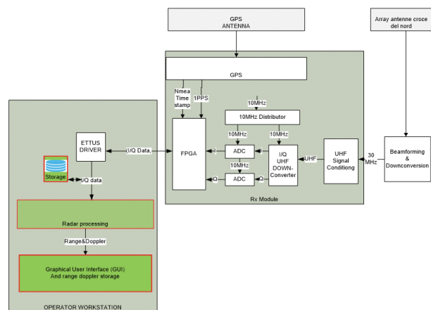
Fig. 4. Receiver architecture
