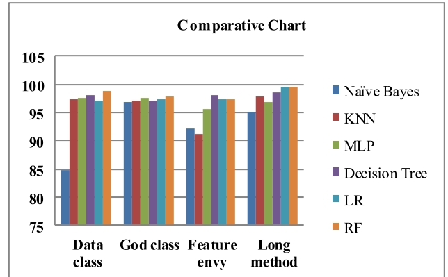
FIGURE 10. Comparison graph of accuracy among six machine learning techniques with four code smell datasets.
