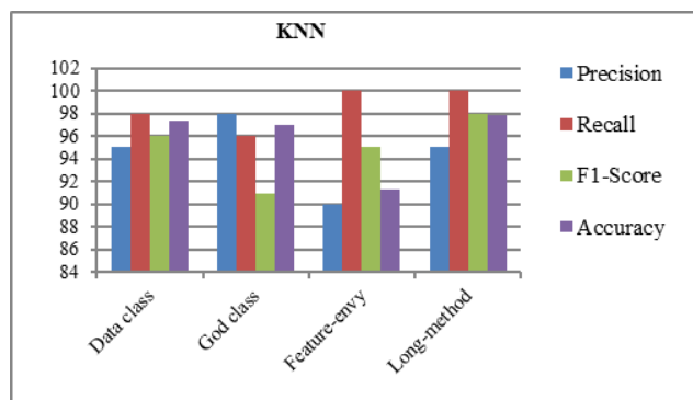
FIGURE 5. Comparative performance bar chart of all datasets with KNN technique.
