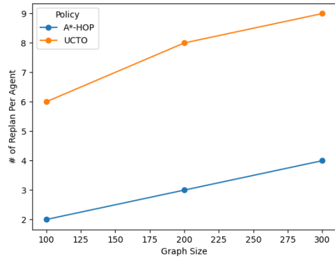
(b) Euclidean graphs
