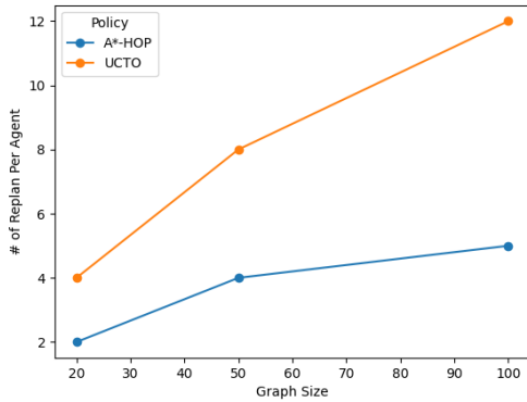
(a) Delaunay graphs
