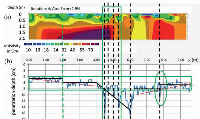
Fig. 6 Studying a fault structure: (a) ERT section. (b) PreP profile. Dotted lines denote the fractures on basis of the PreP results. Green rectangle delineates the interpreted fracture zone. Black and red lines show the average values in the given zone
