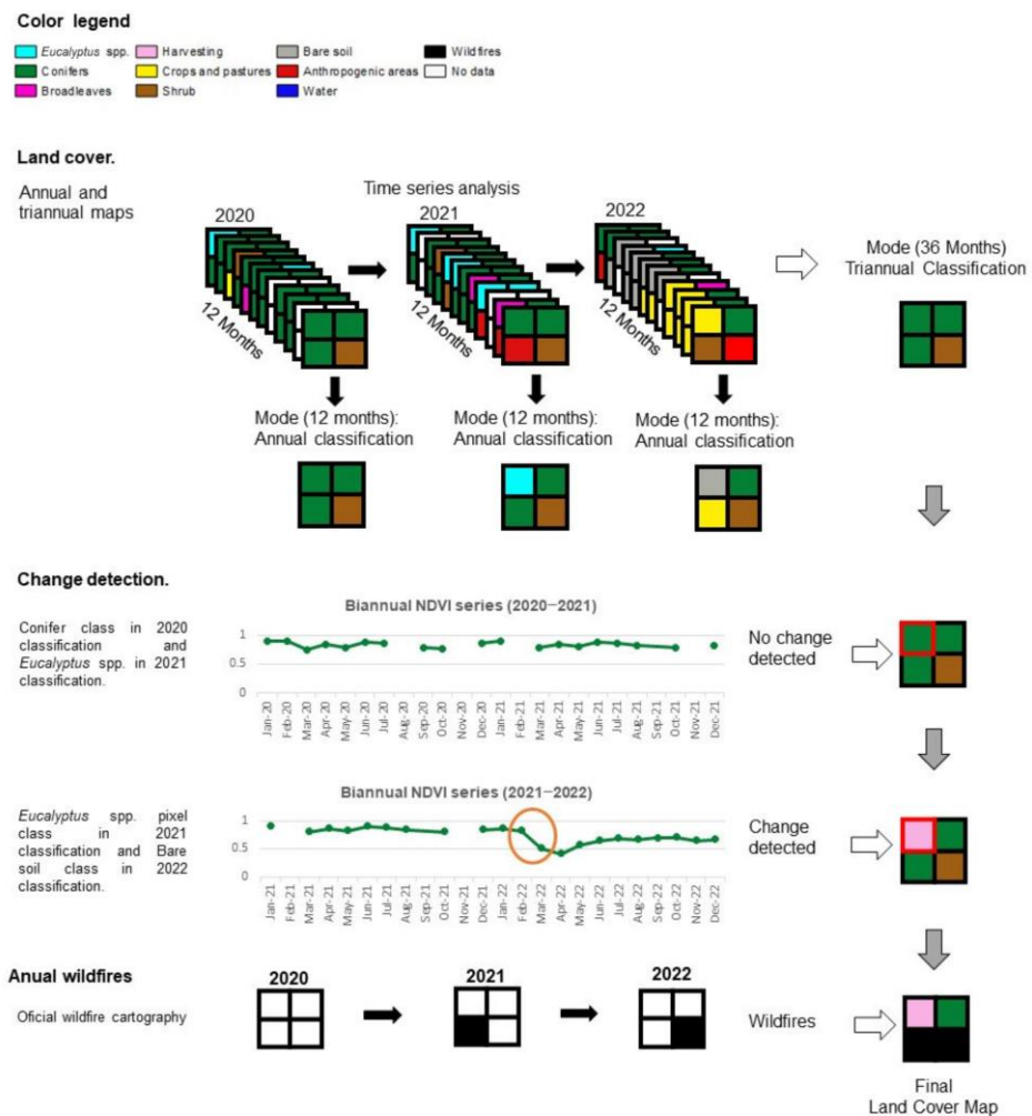
Figure 4. Methodology used to obtain the ultimate forest-oriented land cover map. The orange circle marks a drop in the NDVI due to a change in forest cover. The orange circle marks a drop in the NDVI due to a change in forest cover.
