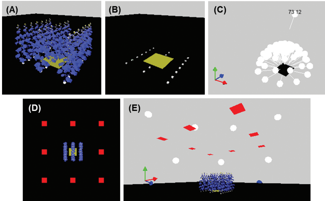
Figure 3. Virtual canopy and light model in the dynamic plant model using RT. (A) A virtual cucumber canopy at a plant density of 1.33 plants per \text{m}^2 . The canopies used in the simulations consisted of 21 plants arranged in three north-south oriented rows and seven plants per row. The central three plants in the middle row were sampled for output. (B) Location of rockwool cubes (white squares, height 6.5 cm), from which single virtual plants were grown to form a virtual canopy. A light sensor (yellow square) covering a ground area of three plants was positioned under the canopy 3.5 cm above the rockwool cubes (thus the middle three rockwool cubes are covered). This light sensor had 0 % transmittance and a reflectance similarly to the ground in the corresponding greenhouse experiments. (C) Light model consisting of one direct and 72 diffuse light sources. Blue y -axis indicates south in the 3D scene. (D) Positions of eight light sensors (each had a size of 1 \text{ m}^2 , red squares) for adjusting incident light, viewed from the top and (E) viewed from a side perspective. These eight sensors had 0 % reflectance and 99.9 % transmittance of light and thus negligible interaction with the virtual scene. The yellow and red coloration of the light sensors shown was only for the visualization. The greenhouse structure was not explicitly considered.
