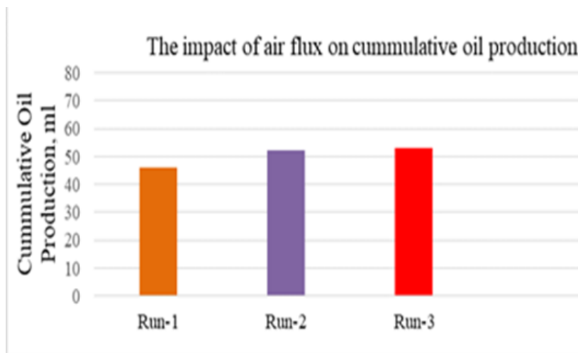
Fig. 3. Cumulative oil production with various air fluxes
