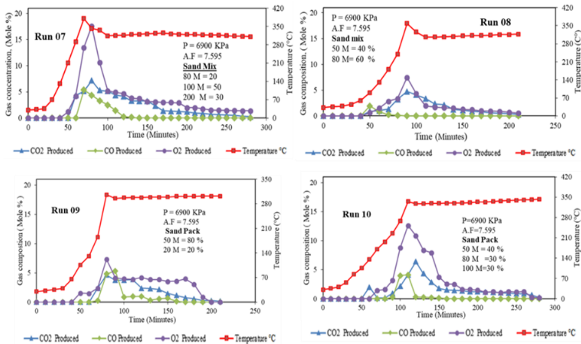
Fig. 6. Temperature and gas composition vs. time at different sand packs
