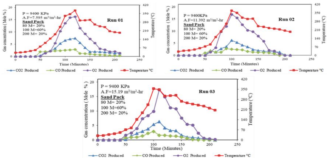
Fig. 2. Temperature and gas composition vs. time at different air fluxes of 7.65, 11.392 and 15.595 Sm 3 /m 2 -hr
