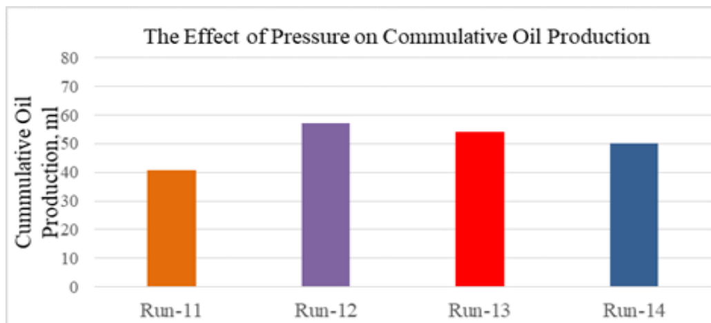
Fig. 9. Cumulative oil production at different pressures of 6900, 7300, 8050 and 9400 KPa
