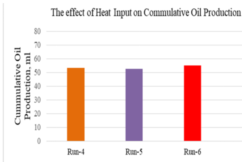
Fig. 5. Oil production with varied heat additions
