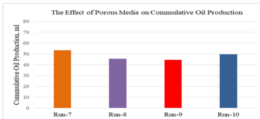
Fig. 7. Oil production with varied mesh sizes properties
