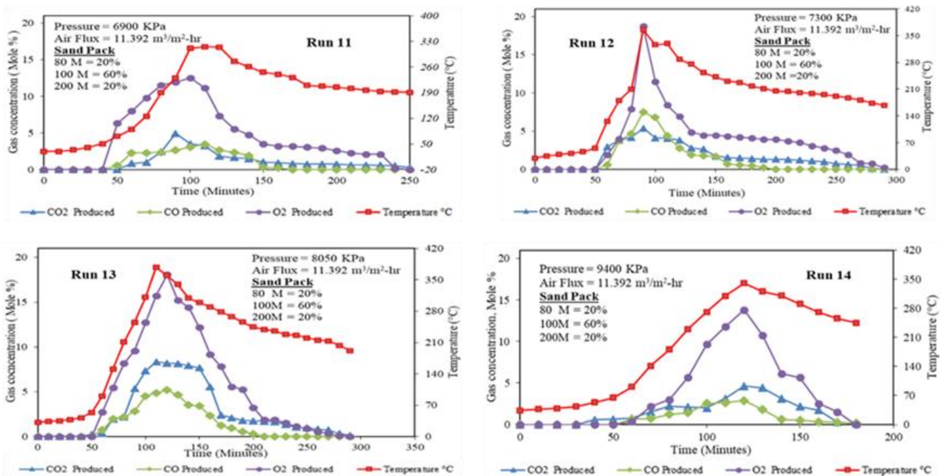
Fig. 8. Gas Composition and temperature vs. time at different pressures of 6900, 7300, 8050 and 9400 KPa
