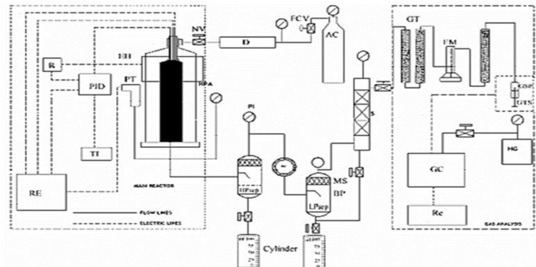
Fig. 1. Air injection experimental systems
