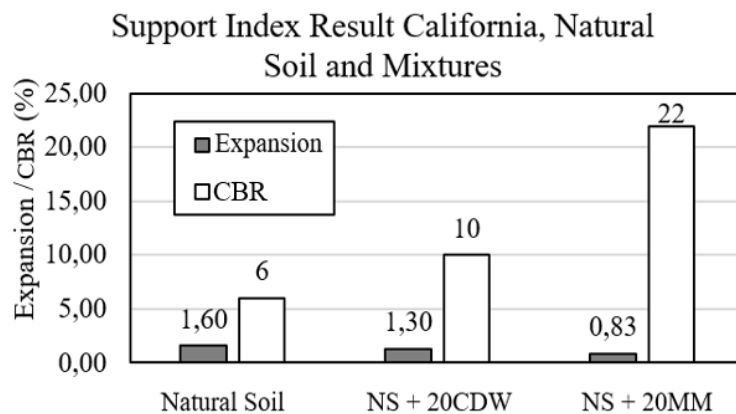
Figure 7. Support Index Result California, Natural Soil and Mixtures.
