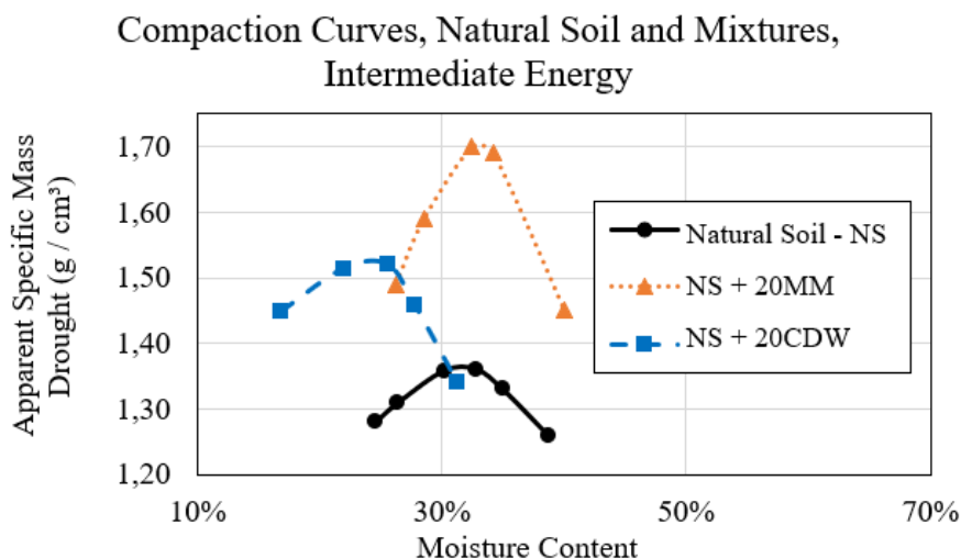
Figure 5. Compaction Curves, Natural Soil and Mixtures, Intermediate Energy. Source: Own Author
