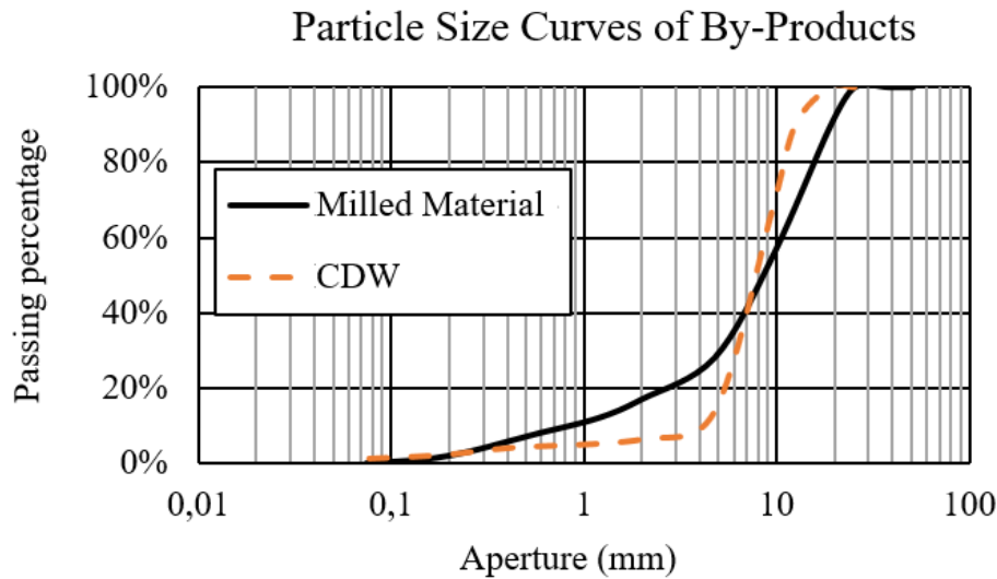
Figure 4. Grain size curves of the by-products. Source: Own Author
