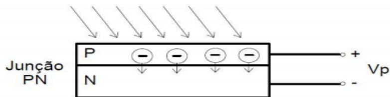
Figure 1. Simplified Scheme of a Photovoltaic Cell.
