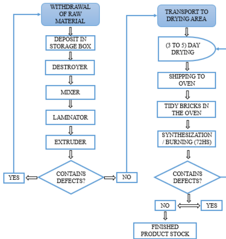
Figure 4: Flowchart of the production process of the pottery studied. Source: Own author.
