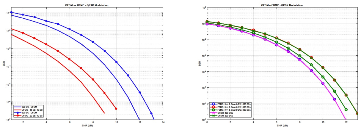
Figure 8. The comparison UPMC and FBMC vs CP-OFDM.
