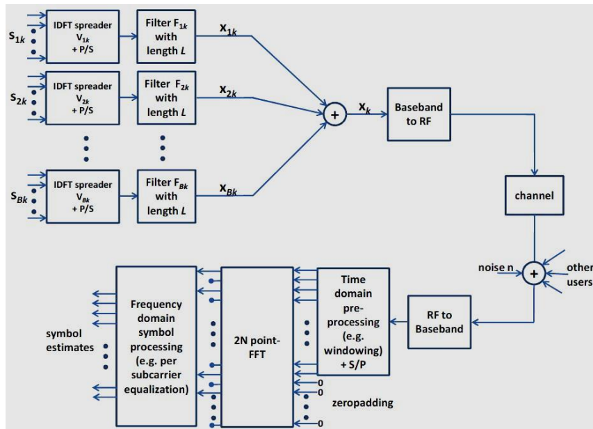
Figure 4. UPMC transceiver.
