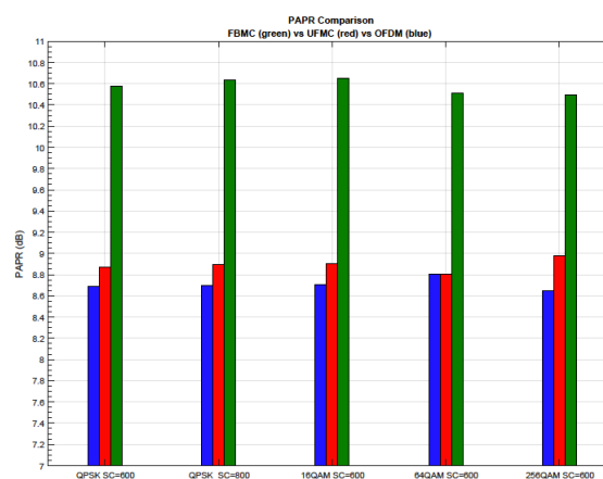
Figure 9. PAPR comparison between CP-OFDM, UPMC, and FBMC.
