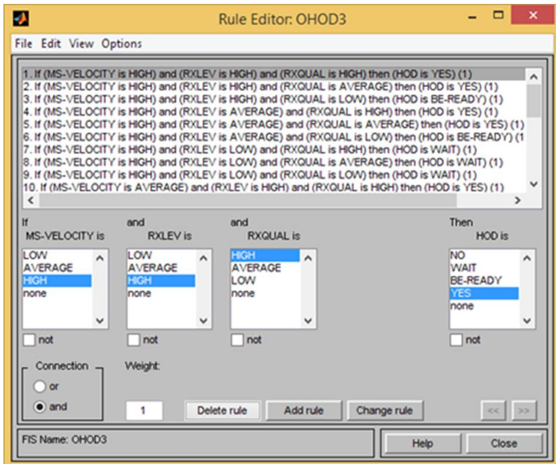
Figure 4c: Some Rules for 3-input FIS
