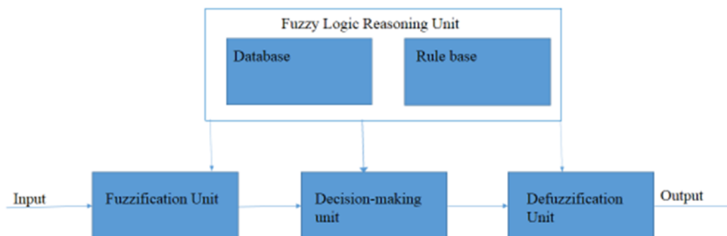
Figure 2: The Basic Structure of a Fuzzy Inference System [17]
