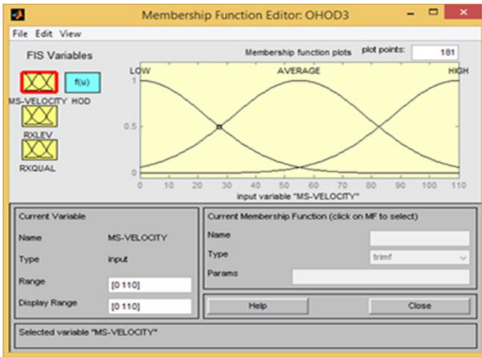
Figure 4b: MFs for MS Velocity
