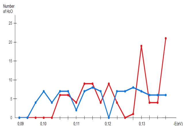
Fig. 6. The number distribution of water molecules in the sample (red color) with 1% suspension of C. vulgaris in 24.5% heavy and 75.5 % deionized water and a control sample (blue color) with 24.5% heavy and 75.5 % deionized water according to the energies of hydrogen bonds.
