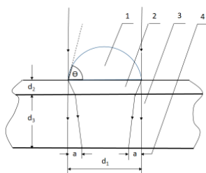
Fig. 2. Design of hard surface for study of wetting angle during the evaporation of water drops. 1 – water drop, 2 – mylar, 3 – glass base, 4 – width of the optical refraction ring.
