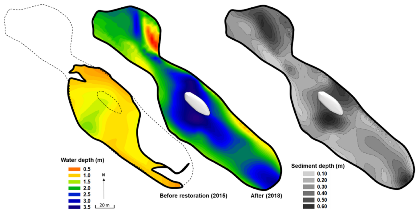
FIGURE 3 Changes in the morphometry of Lake Mustijärv (Estonia). High external loads recharged the sediment nutrient pool soon after sediment removal, partly due to intensive cleaning of an upstream streambed (from Kiani et al., 2020).
