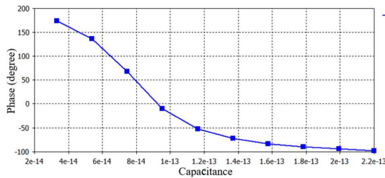
Fig. 9. Simulation results of the varactor diode capacitance versus phase variation
