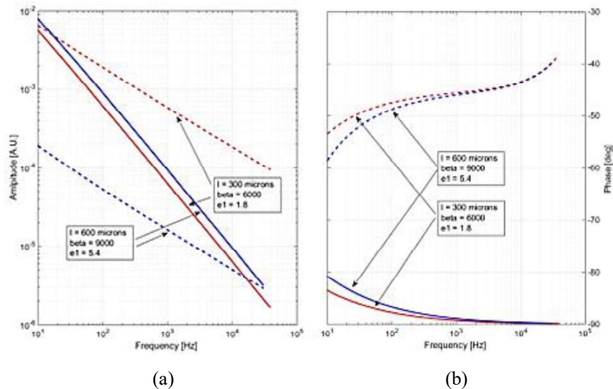
Figure 1. The influence of different values of absorbance ( e_1 ) on amplitude (a) and phase (b) of surface temperature variations of the examined sample (illuminated side given in full, backside in dotted lines) [3].
