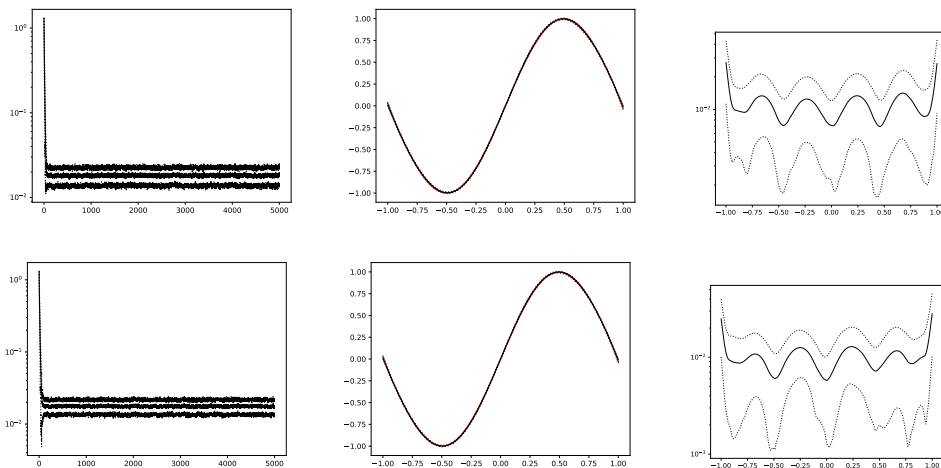
Figure 4: Estimation results of the polynomial regression problem using stochastic gradient descent with constant learning rate \eta = 0.1 (top row) and a version of stochastic gradient descent that uses the implicit midpoint rule (bottom row). The figures depict the mean over 100 runs (black solid line), mean \pm standard deviation (black dotted line). Left column: trajectory of the rel_err over time; centre column: comparison of \Theta (solid red line) and estimated polynomial; right column: estimation error in terms of abs_err .
