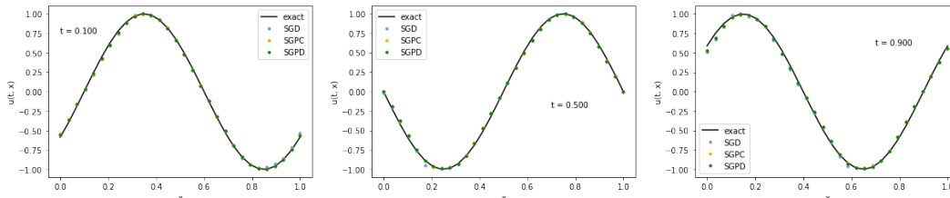
Figure 9: The plots of the solutions at time t = 0.1, 0.5, 0.9 . We evaluate the models at 30 uniformly sampled points. For each method, the predicted values are taken by averaging over the predicted values from the best models (the model that achieves the lowest training loss within the 600 iteration steps) in 30 random experiments. The black curve is the theoretical solution.
