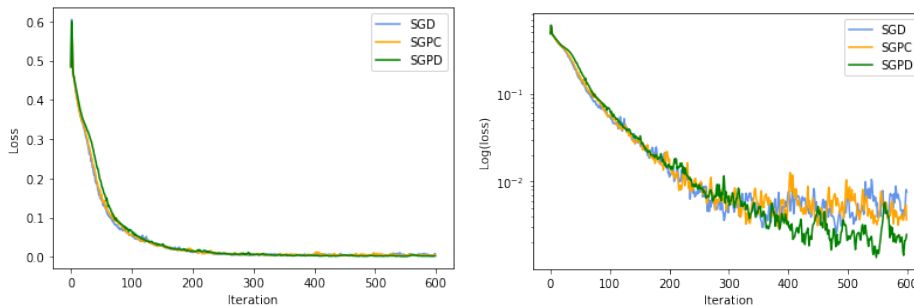
Figure 8: The plots of the loss vs iteration and its log scale for SGD, SGPC, and SGPD. The losses are obtained by averaging over 30 random experiments.
