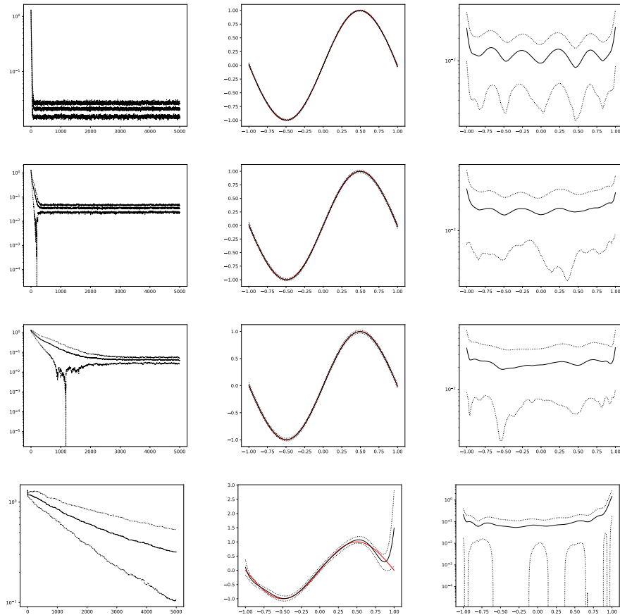
Figure 6: Estimation results of the polynomial regression problem using the stochastic gradient process with pure jump index process with \lambda = 10 (first row), \lambda = 1 (second row), \lambda = 0.1 (third row), and \lambda = 0.01 (fourth row). The figures depict the mean over 100 runs (black solid line), mean \pm standard deviation (black dotted line). Left column: trajectory of the rel_err over time; centre column: comparison of \Theta (solid red line) and estimated polynomial; right column: estimation error in terms of abs_err .
