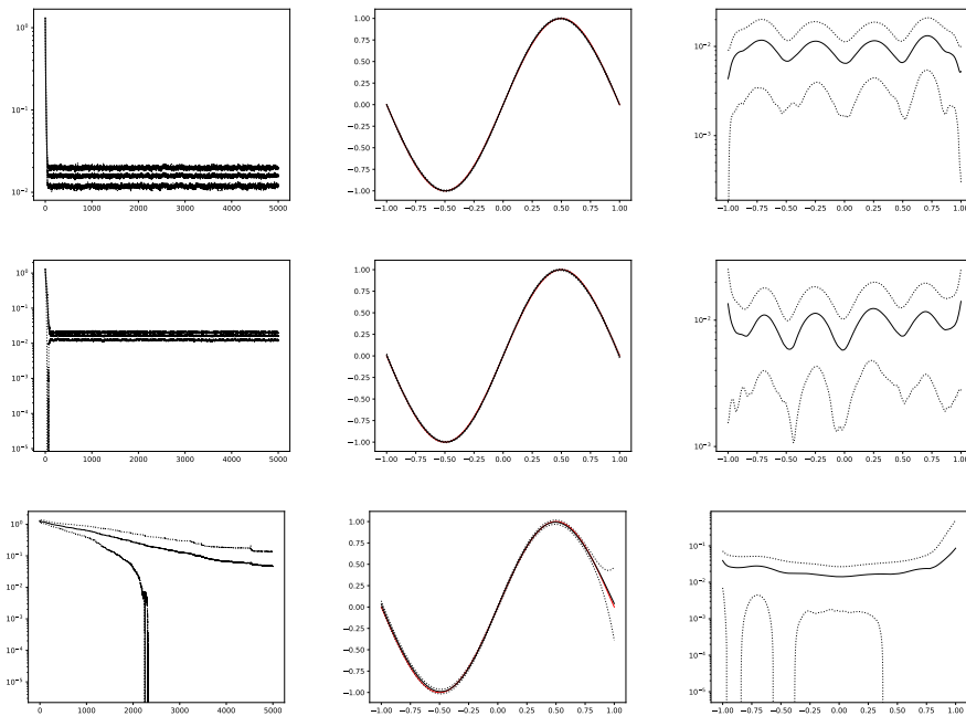
Figure 5: Estimation results of the polynomial regression problem using the stochastic gradient process with reflected Brownian motion process with \sigma = 5 (top row), \sigma = 0.5 (centre row), and \sigma = 0.05 (bottom row). The figures depict the mean over 100 runs (black solid line), mean \pm standard deviation (black dotted line). Left column: trajectory of the rel_err over time; centre column: comparison of \Theta (solid red line) and estimated polynomial; right column: estimation error in terms of abs_err .
