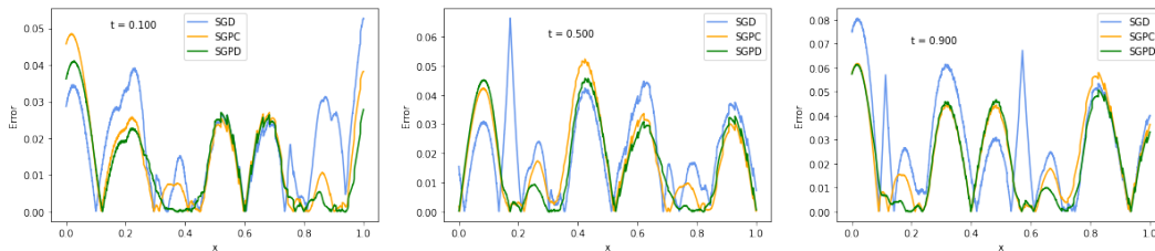
Figure 10: The plots of the test error at time t = 0.1, 0.5, 0.9 . We evaluate the models at 2000 uniformly sampled points. For each method, the predicted values are taken by averaging over the predicted values from the best models (the model that achieves the lowest training loss within the 600 iteration steps) in 30 random experiments. At each point x , the error calculated by taking the absolute value of the difference between the predicted value and the true solution.
