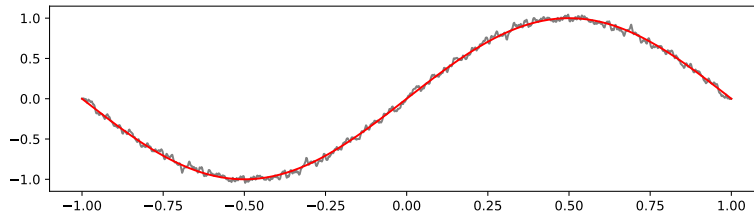
Figure 3: True function \Theta (red) and noisy observation g (grey) in the polynomial regression example.
