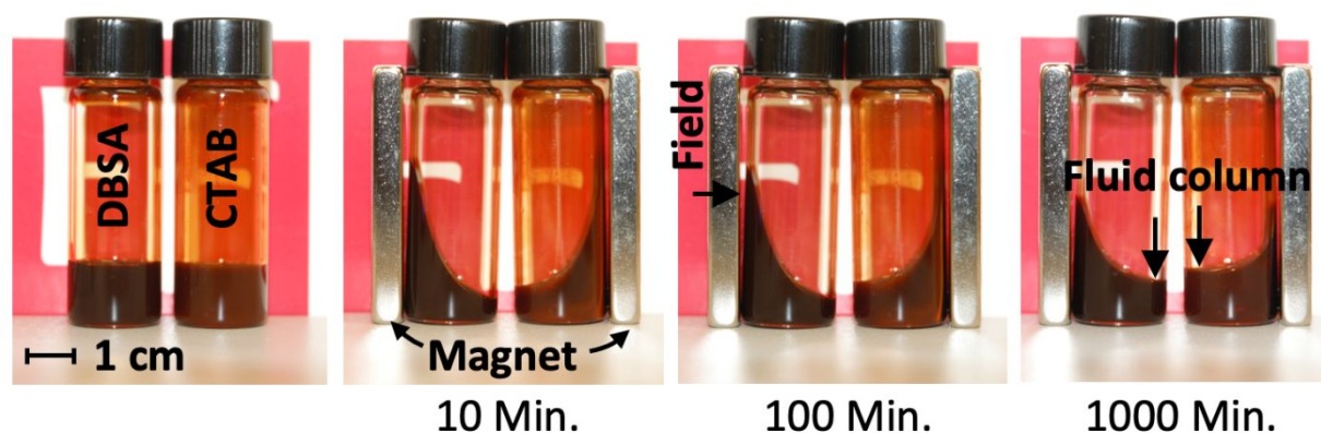
Figure 9: Experimental destabilization times of DBSA/BHF and CTAB/BHF ferrofluid (40 mg/ml) exposed to a permanent magnetic field (0.3 T).
