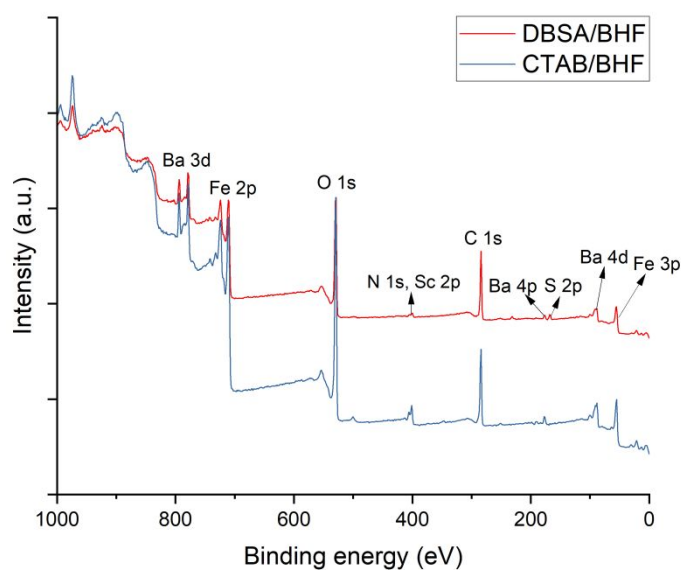
Figure 5: XPS spectra of dry DBSA and CTAB coated BHF nanoparticles
