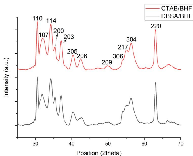
Figure 4: XRD patterns of DBSA/BHF and CTAB/BHF coated Barium Hexaferrite with labelled crystallographic planes corresponding to hexagonally crystal symmetry (space group P6_3/mmc ) BHF nanoparticles.
