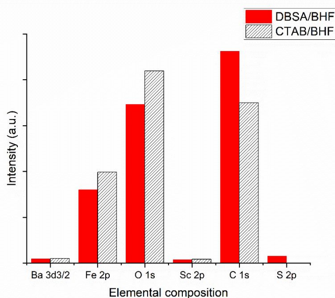
Figure 6: Surface elemental composition of dry DBSA and CTAB coated BHF nanoparticle powders.
