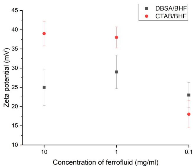
Figure 8: Zeta potential data for the DBSA/BHF ferrofluid in butanol and CTAB/BHF in ethylene glycol with standard deviation for zeta potential-measurements.
