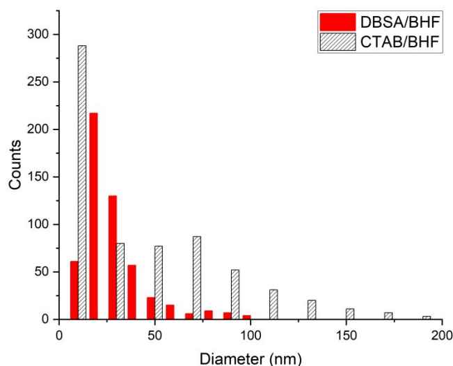
Figure 2: Diameter distribution of the nanoplatelets produced at 190 °C: CTAB/BHF dispersed in ethylene glycol and DBSA/BHF dispersed in 1-butanol.
