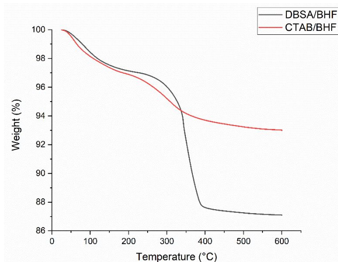
Figure 7: Thermal decomposition (TGA) curves of DBSA/BHF and CTAB/BHF powder samples heated from 25 °C to 600 °C at 10 °C/min in air.
