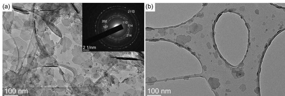
Figure 1: TEM images of the nanoplalelets coated with: (a) CTAB dried from ethylenegylcol and (b) DBSA dried from 1-butanol. Insertion in panel (a) shows SAED with indices corresponding the barium hexaferrite structure, space group P6_3/mmc (194).
