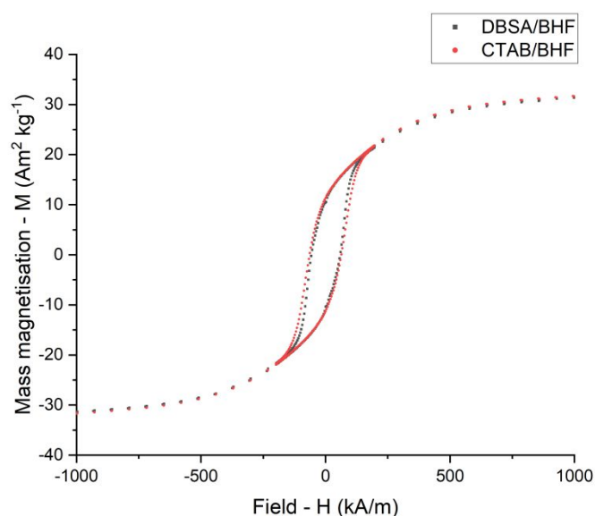
Figure 3: Mass magnetisation – M against Applied Field – H of Barium Hexaferrite nanoparticles coated with DBSA and CTAB.
