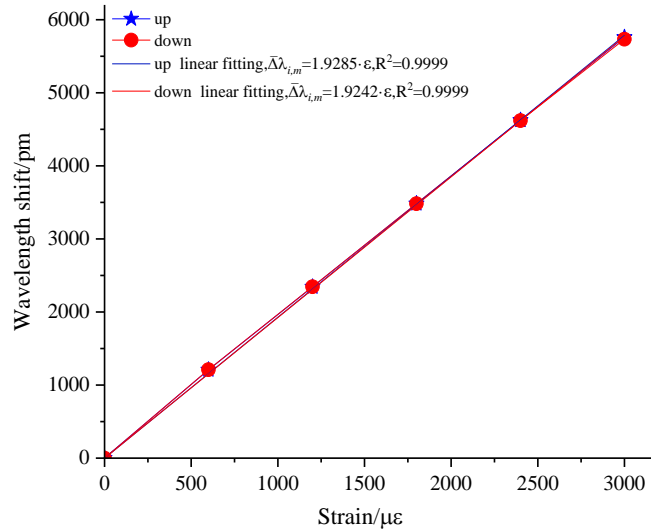
Fig. 5. Fitting curves of strain grating \Delta\bar{\lambda}_i
