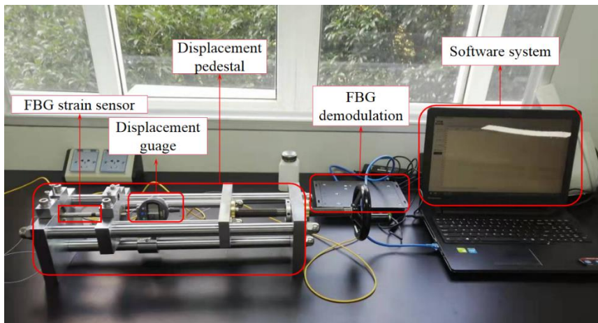
Fig. 3. Strain sensitivity test device
