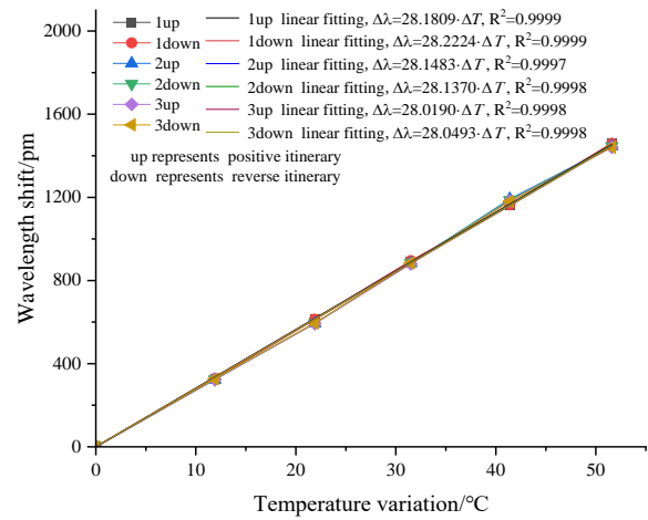
Fig. 9. Fitting curves for temperature sensitivity K_{T-T}
