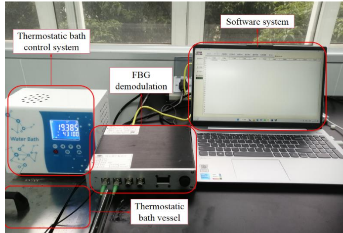
Fig. 7. Temperature compensation test device
