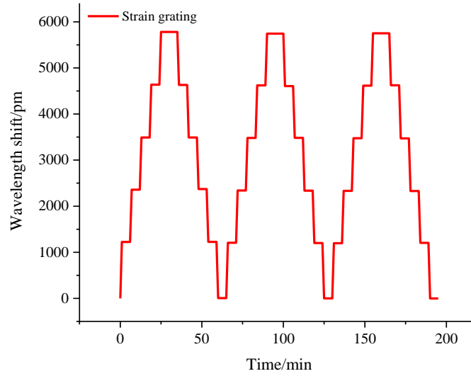
Fig. 6. Wavelength shift-time curve for three repetitions of the sensor
