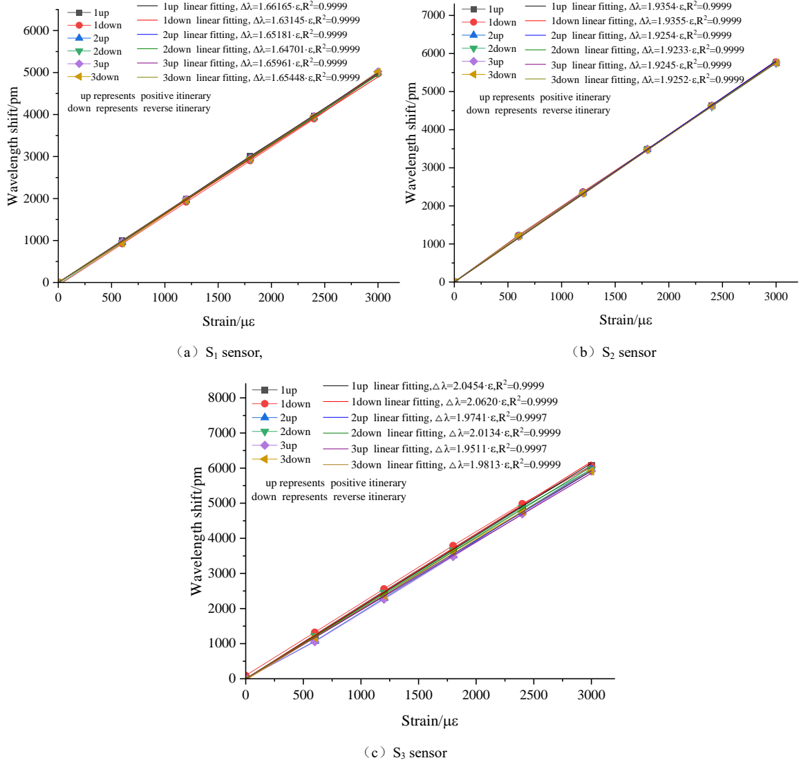
Fig. 4. Fitting curves of strain sensitivity coefficient K_{\epsilon-S} for strain grating
