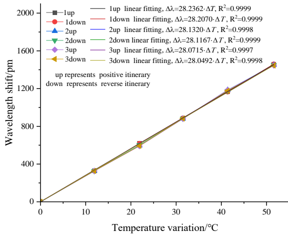
Fig. 8. Fitting curves for temperature sensitivity K_{T-S}
