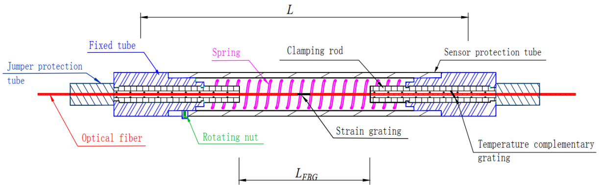
Fig. 1. FBG sensor structure diagram
