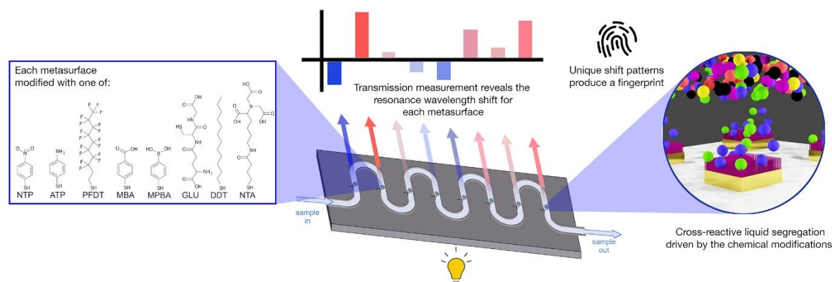
Figure 1. Schematic of the sensor concept. Eight metasurfaces are linked by a microfluidic channel. Each metasurface is modified with a different surface chemistry, providing partial-selectivity to the components in the water sample. Thus, each metasurface experiences a unique refractive-index environment, shifting its resonance wavelength value. By tracking the combination of resonance shifts we build a fingerprint for each sample.
