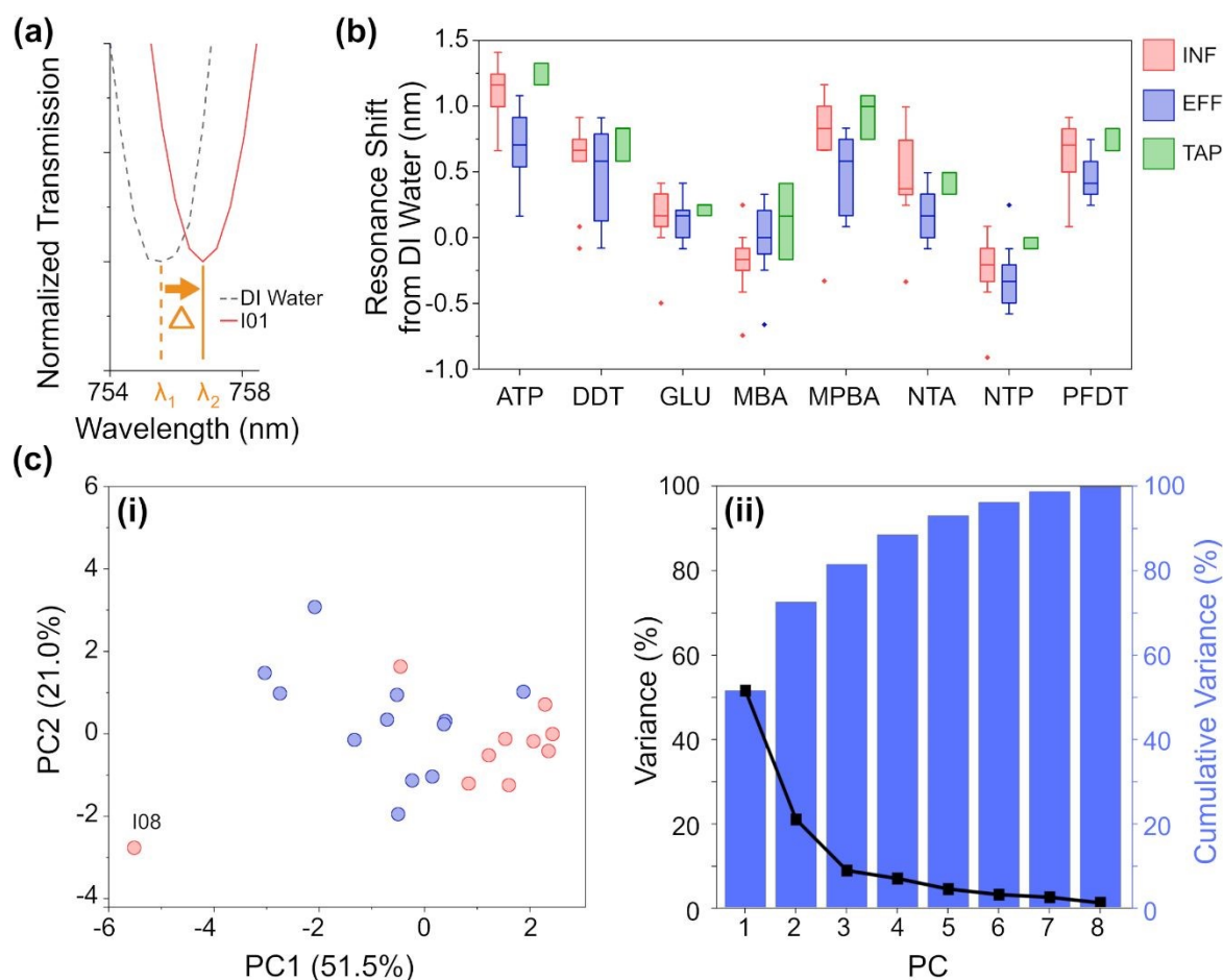
Figure 3. (a) Example of a resonance redshift from DI Water (ATP chemistry, sample I01). (b) Resonance shift from DI Water of each NTB grouped by water sample type. (c) PCA of the resonance shift (average shift from DI Water) for INF and EFF: (i) Scatterplot of the first and second principal components and (ii) a plot of the variance and cumulative variance as explained by each PC.
