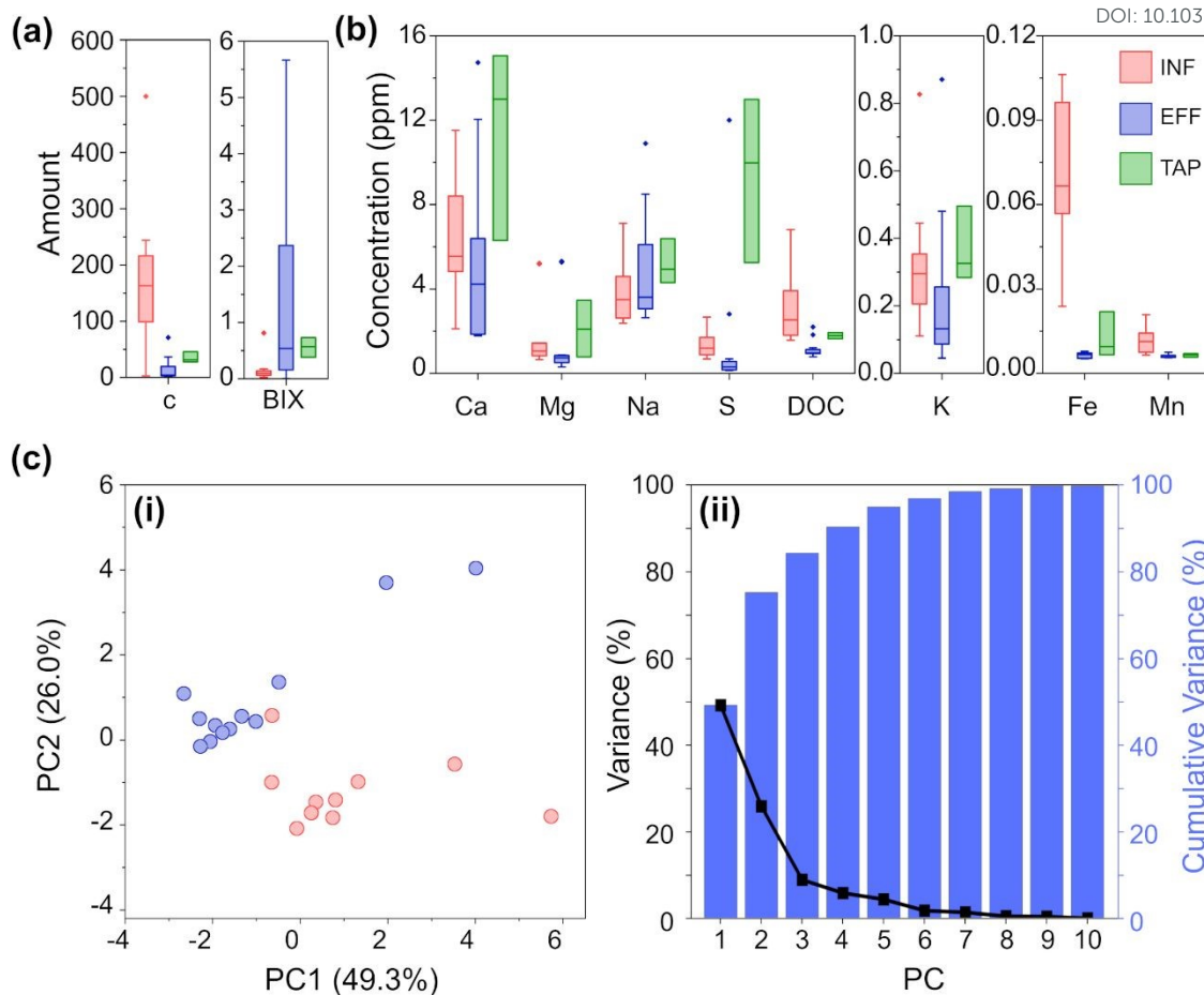
Figure 2. (a) FEEM analysis grouped by water sample type for peak C and bix. (b) ICP-OES and DOC analyses grouped by water sample type (concentrations are in ppm). (c) PCA of the analytical chemistry results for INF and EFF: (i) Scatterplot of the first and second principal components (PC) and (ii) a plot of the variance and cumulative variance as explained by each PC.
