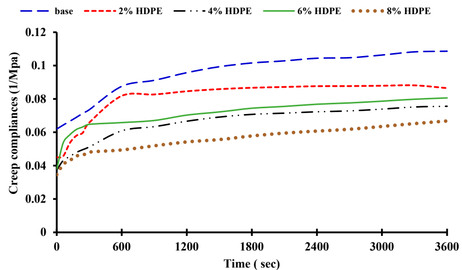
Figure 12. Creep compliances with time for high-density polyethylene-modified mixtures.
