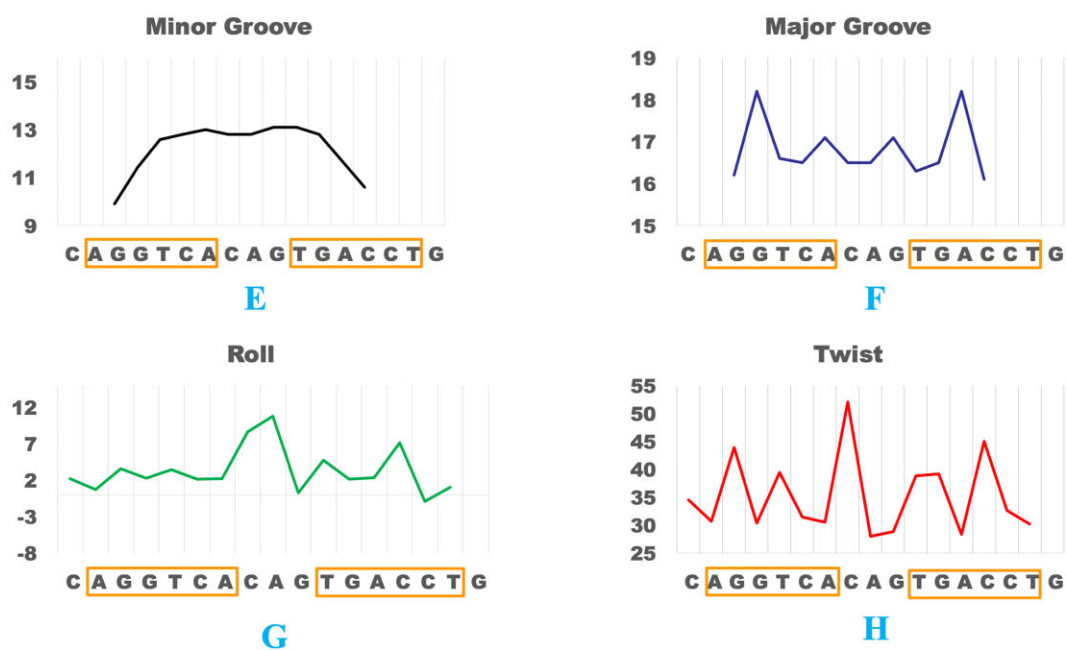
Figure 6. (A–D) DNA geometrical parameters of the emberRE/IR3 DNA bound by ER \alpha , showing the (A) minor groove width, (B) major groove width, (C) roll, and (D) twist parameters. (E–H) DNA geometrical parameters of the ERE-IR3 bound by ER \alpha DBD homodimer (PDB code 1HCQ, (38)), showing the (E) minor groove width, (F) major groove width, (G) roll and (H) twist parameters.
