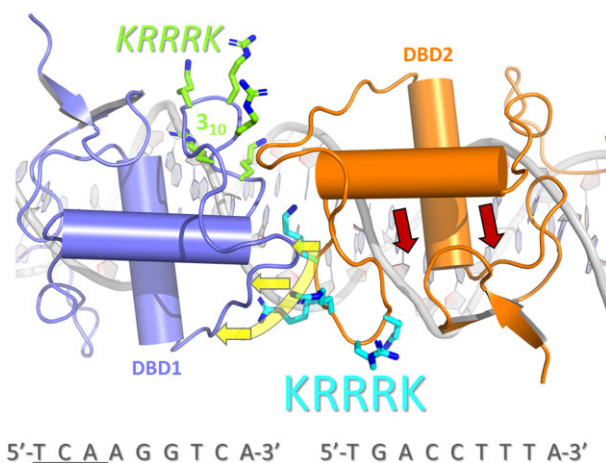
Figure 7. A representation of the ERR \alpha DBD/ERRE complex, summarizing our main structural observations. The dimerization interface of ERR \alpha DBD homodimer is made by interactions between the D box of each subunit. Furthermore, it is reinforced by the presence of an extended interaction area arising from the KR-box region of DBD2 that unfolds as a loop and interacts with the dimerization region of DBD1, as indicated by yellow arrows. The dimerization interface is asymmetric with different KR-box conformations for the two subunits (highlighted by the lemon green and teal colours) and it is required for proper stabilization of the DBD homodimer on DNA (as suggested by the red arrows), suggesting the importance of the DNA, which acts as allosteric driver in accommodating the receptor in a fully functional state suitable for gene expression regulation. The subunit bound to the extended half-site, DBD1, is shown in blue colour and DBD2 is shown in orange colour.
