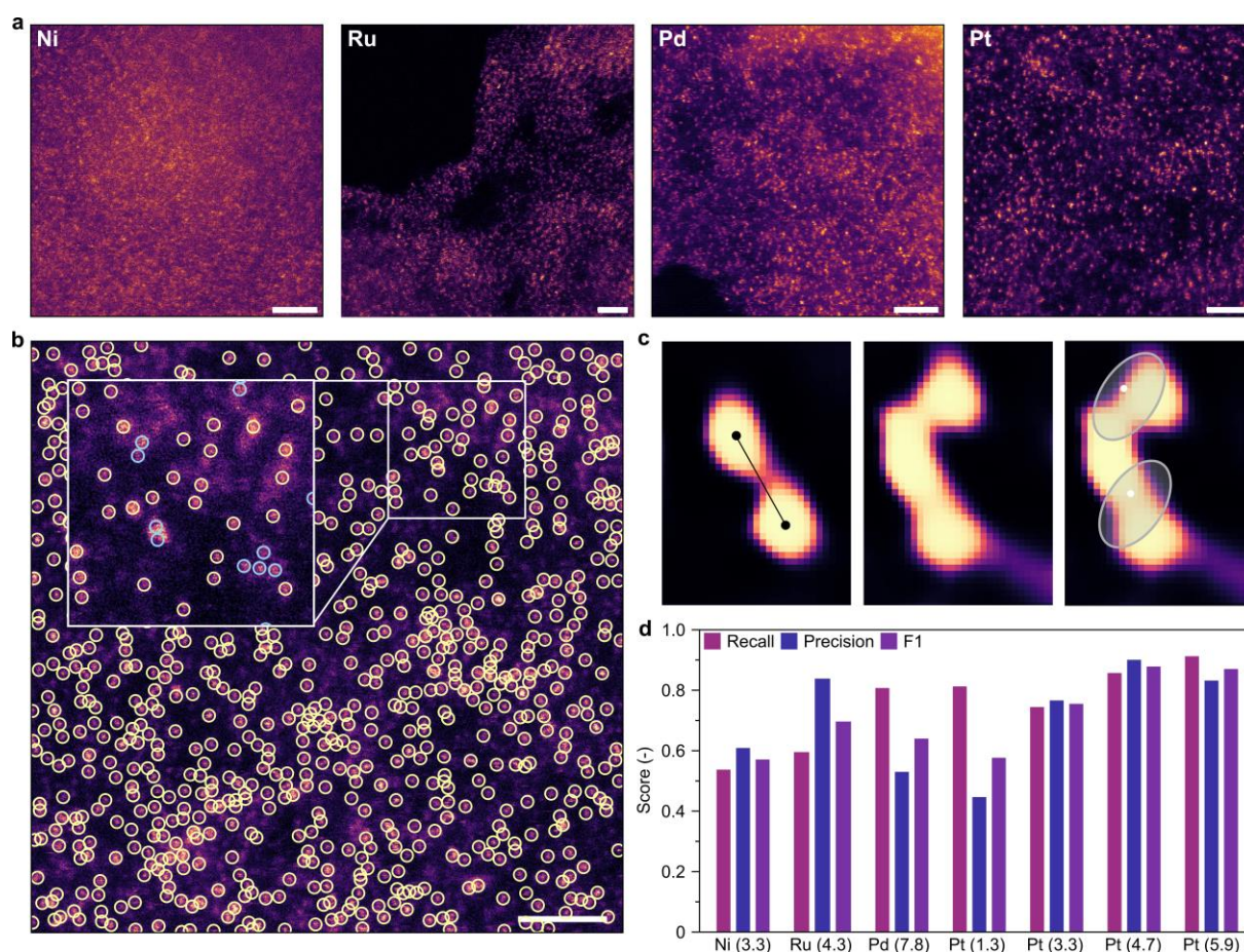
Figure 2. a , AC-STEM images of distinct UHD-SACs, illustrating the variation in contrast of the metal centers with the NC host material. All scale bars correspond to 2 nm. b , AC-STEM image of Pt 1 /NC SAC with machine learning-detected atoms overlaid (yellow circles). The zoom inset highlights potential multimers (blue circles) that require detection and quantification. c , Representative prediction maps generated by the CNN for multimers assigned in b , exemplifying the analysis of interatomic distances (left panel) and, the use of Gaussian mixture model assignments to resolve overlapping features (central and right panels). d , Bar charts illustrating the performance metrics of the machine-learning model compared to manual assignments carried out by a domain expert. The comparison involved images of samples with different metal identities, density (in atoms nm -2 , indicated in parentheses after the metal), imaging resolutions, and measurement conditions. The (GPU accelerated) machine-learning model detections for these test images are produced in minutes, whereas the human-expert assignments took a few hours.
