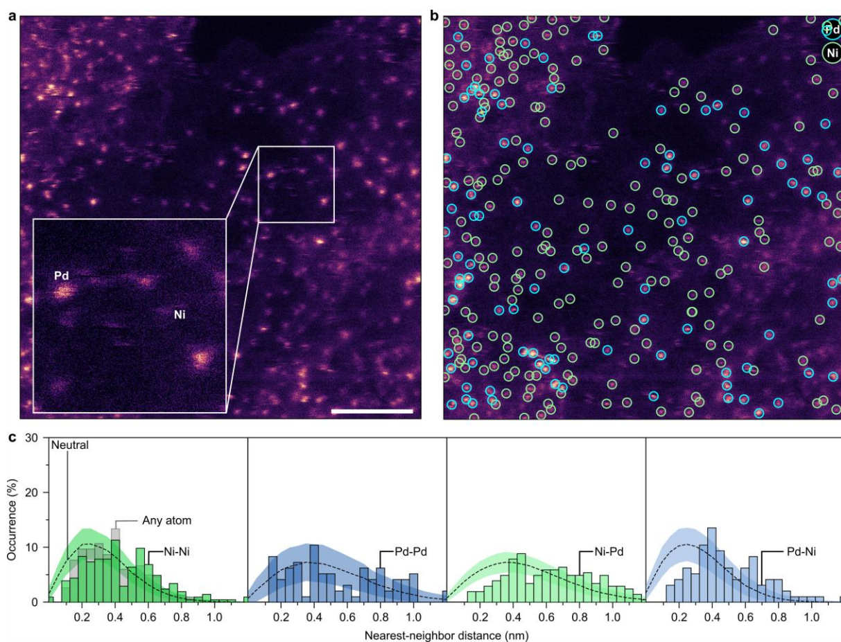
Figure 5. a , AC-STEM image of a bimetallic Ni 1 Pd 1 /NC. The inset illustrates the difference in contrast between Ni and Pd atoms b , corresponding atomic position assignments inferred by the CNN model, where atom chemical identity is predicted by the variational autoencoder latent space clustering approach. c , Breakdown of nearest-neighbor distance distributions when accounting for any possible neighbors (gray) or when considering element-specific pairs in a multimetallic Ni 1 Pd 1 /NC SAC. The
