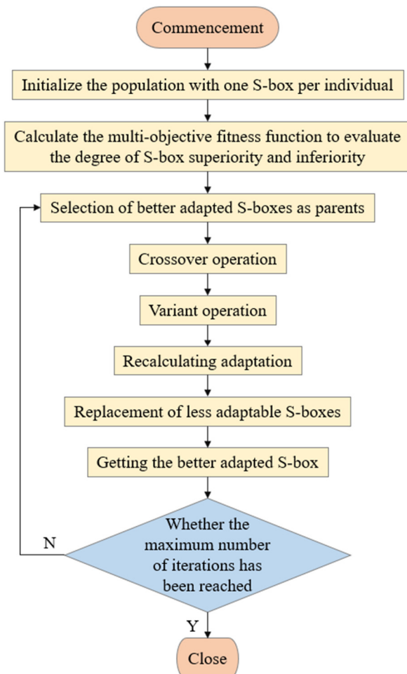
Fig. 3 Genetic algorithm flowchart
