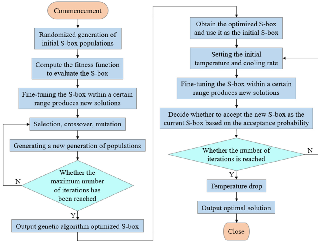
Fig. 5 Flowchart of hybrid algorithm optimization for S-box model
