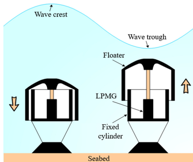
Fig. 8 Schematic diagram of the fundamental operation of an LPMG-based WAS
