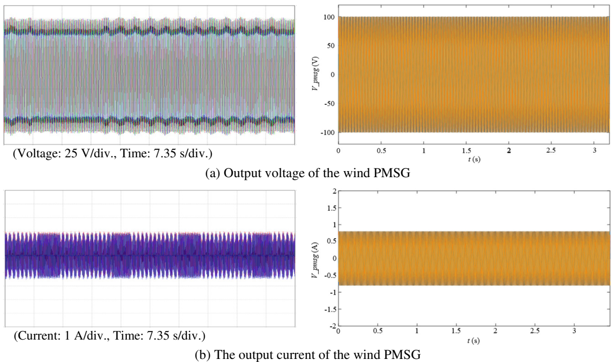
Fig. 12 Comparison: field measurements vs. simulation results for HWWPGS (Fig. 1)
