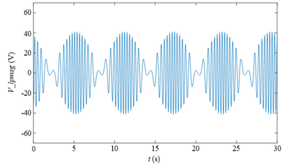
(c) Output voltage of the wave LPMG
