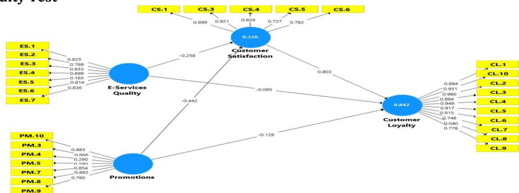
Figure 2. Measurement Model
