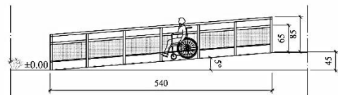
GAMBAR TAMPAK SAMPIING
