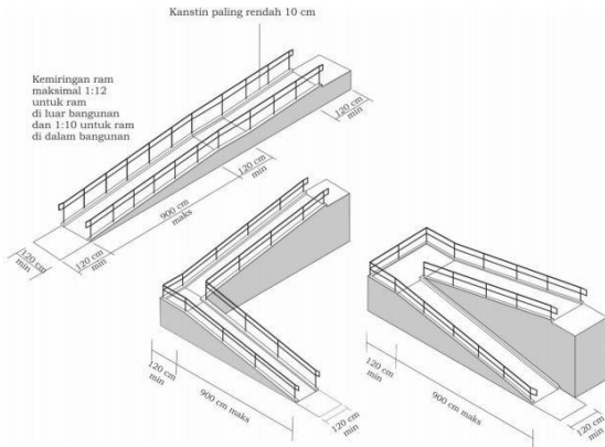
2.9. Gambar denah ram
