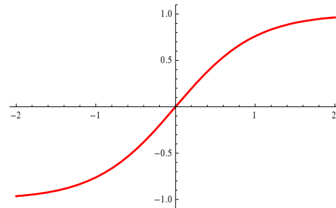
Fig. 1. Antisymmetric sigmoid tangent hyperbolic activation function
