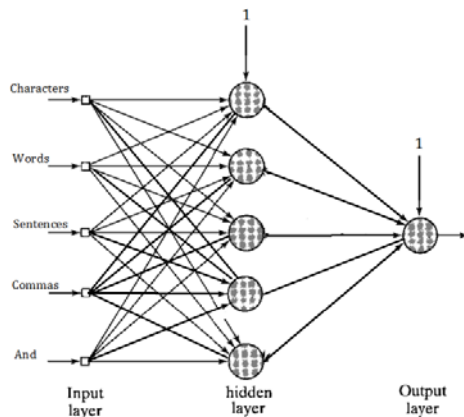
Fig. 3. Signal flow graph of an expert neural network
