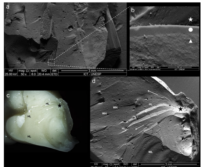
Figure 3 Images of fracture surfaces in stereomicroscope and SEM of anterior and posterior prostheses. Anterior reinforcement sample under 50x magnification (a) and interface between the silica-nylon mesh and composite resin under 2000x magnification (b). White star - nylon; Circle - adhesive; Triangle - composite resin. Posterior sample in stereomicroscope under 7.5x magnification (c) and the same sample in SEM under 50x magnification (d). Black star - fracture origin; Arrow - direction of crack propagation; HL - hackle lines; WH - Wake hackles; WL - Wallner lines.
