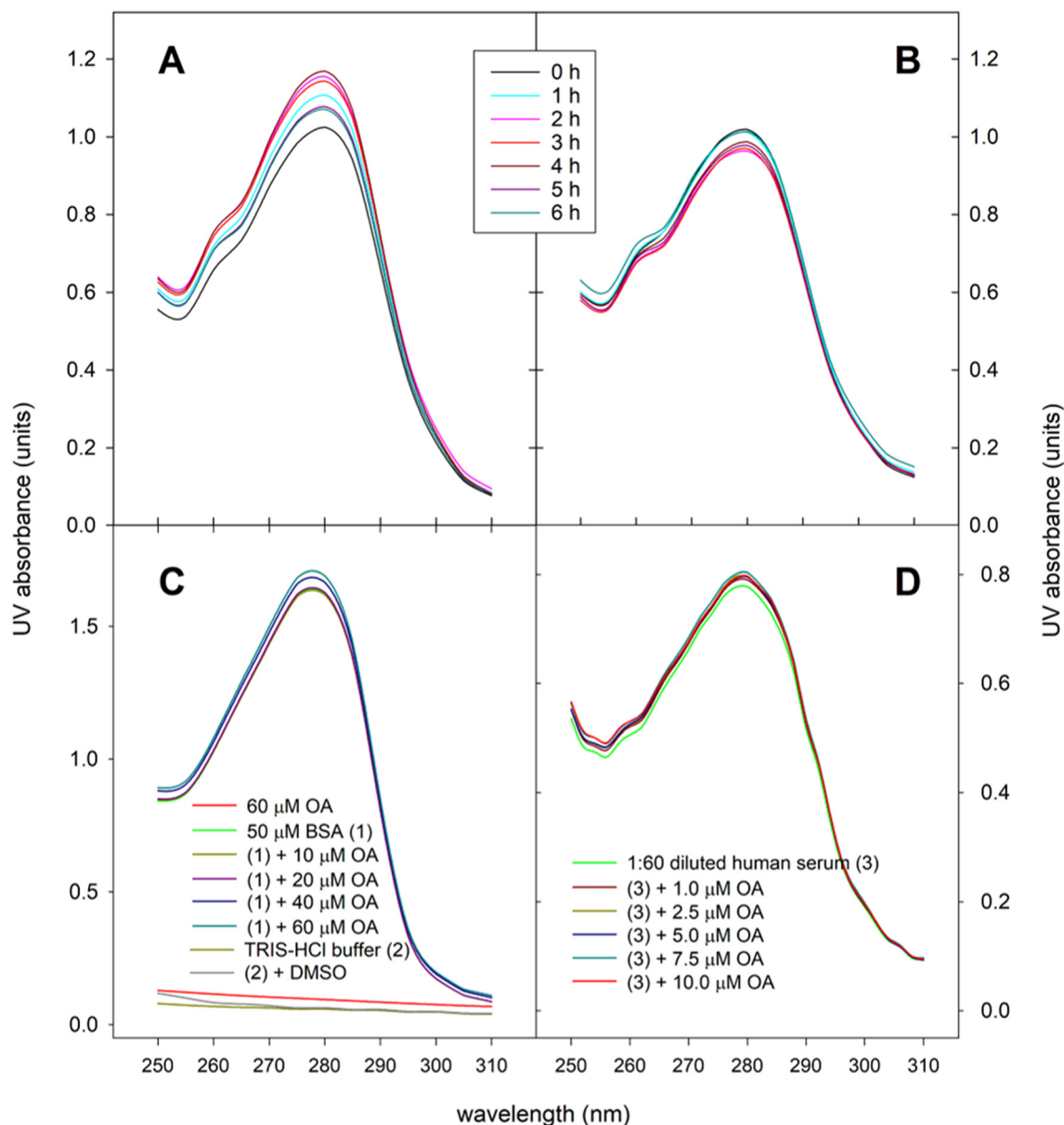
Fig. 4 UV Absorption spectra at 25 °C of serum samples (diluted 1: 50 in 0.1 M Tris-HCl buffer at pH 7.4) obtained before and after the ingestion of the experimental meal containing (A) the OA-enriched olive oil (equivalent dose 30 mg OA) or (B) the control olive oil. (C and D) shows the UV absorption spectra in experiments with standard BSA and blank human serum, respectively, spiked with different concentrations of standard OA.
