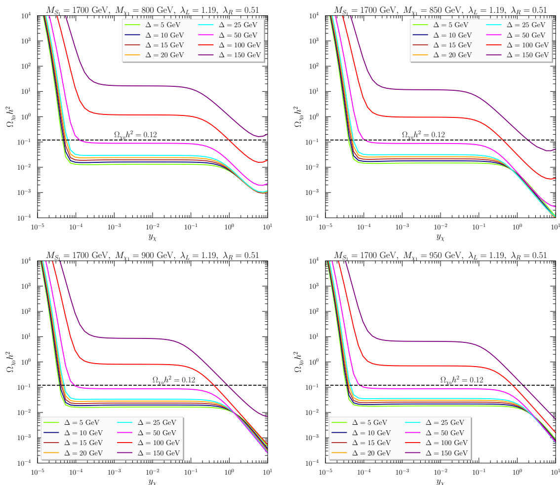
Figure 14. The DM relic abundance as a function of y_{\chi} in BS1 scenarios for M_{S_1} = 1700 GeV, \lambda_L = 1.19 and \lambda_R = 0.51 . We consider four options for the \chi_1 mass consistent with constraints from missing energy searches at the LHC: M_{\chi_1} = 800 GeV (upper left), 850 GeV (upper right), 900 GeV (lower left) and 950 GeV (lower right). The curves in green, navy, sienna, orange, cyan, magenta, red and purple correspond to values of \Delta of 5, 10, 15, 20, 25, 50, 100 and 150 GeV respectively.
