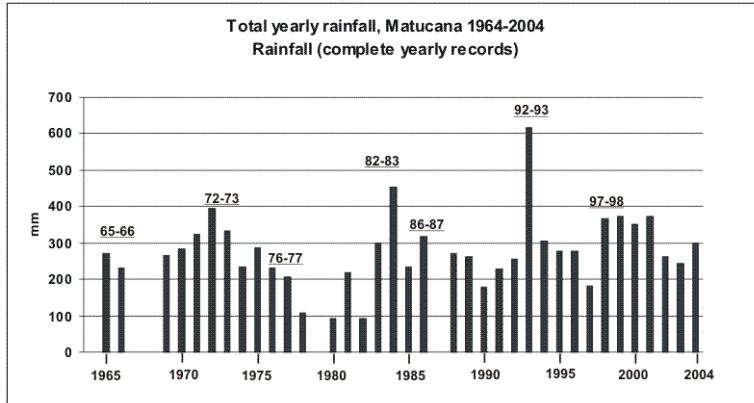
Figure 4. Total yearly rainfall for Matucana Perú. Missing years indicate incomplete data. Underscored numbers indicate El Niño years.
