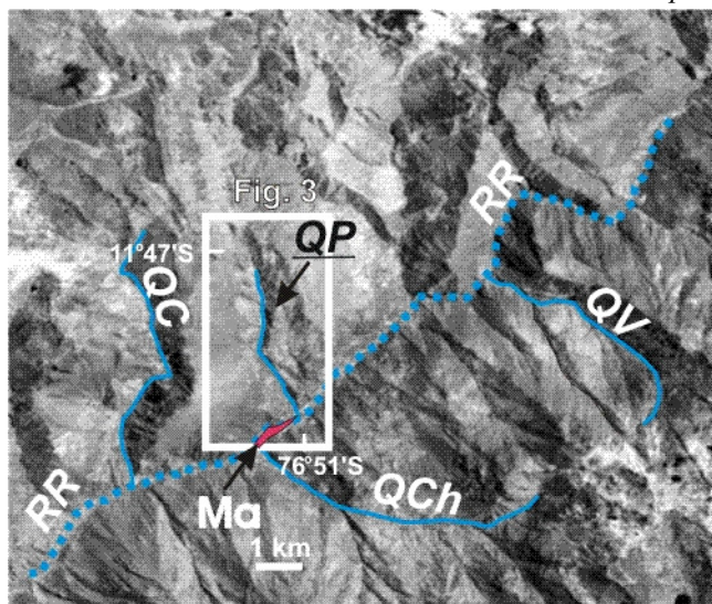
Figure 2. Eros satellite image (2005) of the Payhua- Matucana area: Ma- Matucana, QP- Quebrada Payhua, QV- Quebrada Viso, QCh- Quebrada Chucumayo, QC- Quebrada Collana, RR-Rimac River (Ferrocarril Central and Carretera Central).
