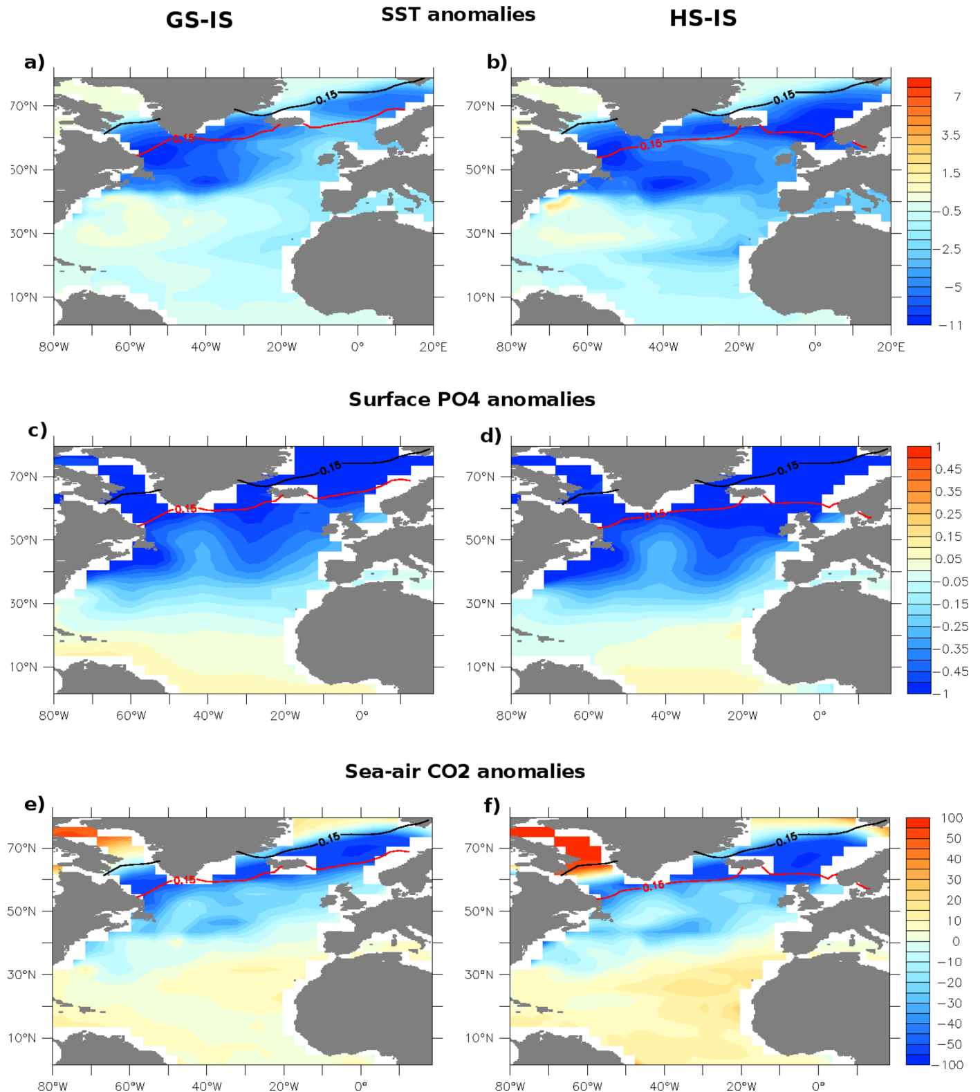
Extended Data Fig. 10 | Simulated climatic and biogeochemical responses to AMOC changes in an Earth system model 18 . Anomalies for (a, b) sea surface temperature (SST; unit °C), (c, d) surface [PO 4 3- ] (μmol/kg), and (e, f) sea-air CO 2 (μatm) for GS-IS (left column) and HS-IS (right column). Black and red curves show sea ice fronts (defined as 15% of sea ice density) during IS and GS/HS,
