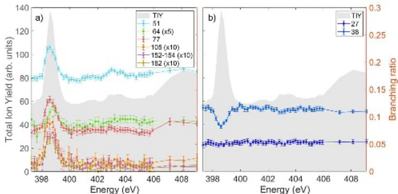
FIG. 10: Total ion yield (TIY, grey shaded area) and branching ratios of the most representative fragments at the N(1s) excitation/ionization region (coloured lines). Panel a) reports examples of fragments with branching ratio increasing at the \pi^* resonance. Panel b) displays examples of fragments either decreasing or unaffected by the core resonant excitation. The entire set of results is reported in Figure IV of the SI. The error bars represent the confidence of the fit.
