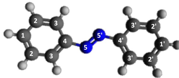
FIG. 1: Azobenzene, AB, (CAS: 103-33-3), m = 182 amu, molecular formula C_6H_5N = NC_6H_5 . The four non-equivalent C atoms on each benzene ring have been labelled 1(1') to 4(4').
