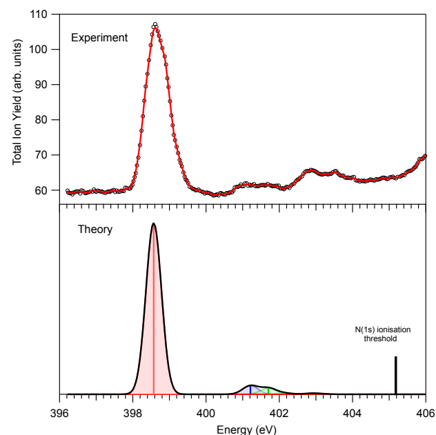
FIG. 8: The nitrogen K-edge NEXAFS spectrum of AB. The experimental data are reported in the top panel as black dots with superimposed 3-point smooth line in red, while the theoretical results convoluted by Gaussian functions of FWHM = 0.7 eV, are depicted the bottom panel. The N(1s) ionization threshold is also reported.
