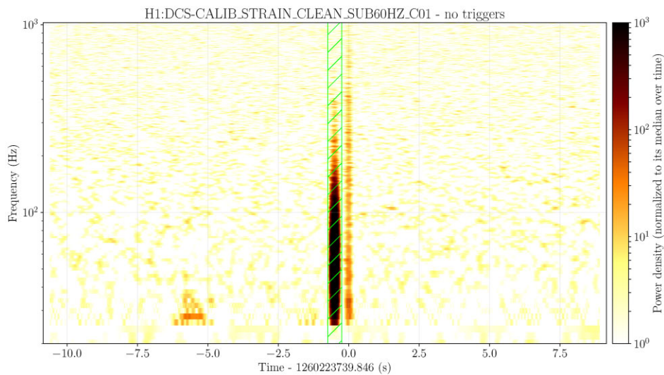
Figure B1. Time–frequency map of the third-ranked PyCBC candidate. This shows the glitch present near to GPS time 1260223739. This represents the kind of quieter glitches that gets skipped in the normal autogating procedures.
