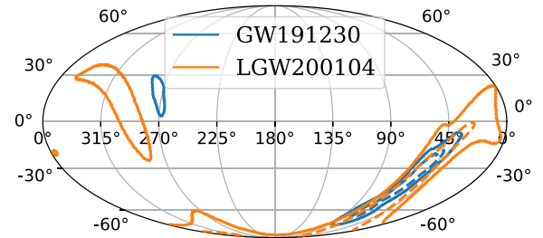
Figure 9. Overlaid LGW200104 and GW191230 skymaps with 90 and 50 per cent CRs.
