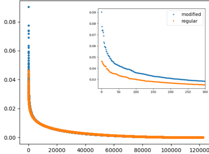
Figure 3: Ordered entries of the entrywise squared absolute values of eigenvector matrices for G_{n,2\lceil\sqrt{n}\rceil} and modified G_{n,2\lceil\sqrt{n}\rceil} with n = 350 (upper right figure is zoomed on the top 300 entries).
