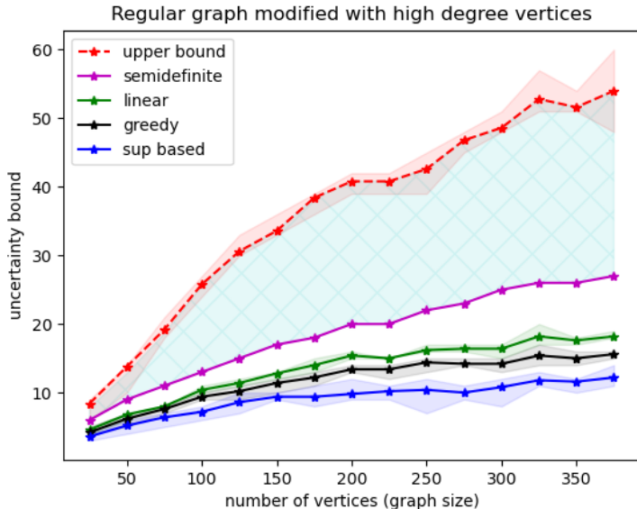
Figure 2: Upper and lower estimates for the uncertainty bound (1) on G_{n,2\lceil\sqrt{n}\rceil} modified by added high-degree vertices, averaged over 5 runs (semidefinite lower bound from 1 run). True value of B is in the cyan region. The bounds suggest sublinear growth of B with n .
