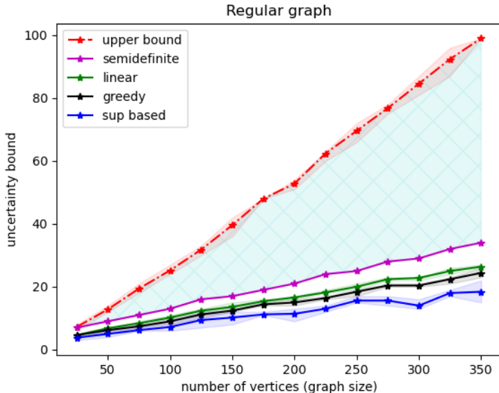
Figure 1: Upper and lower estimates for the uncertainty bound (1) on G_{n,2\lceil\sqrt{n}\rceil} , averaged over 5 runs (semidefinite lower bound from 1 run). True value of B is in the cyan region. All the bounds suggest linear growth of B with n .
