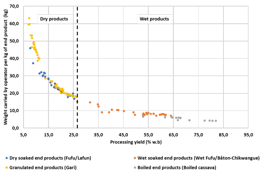
Figure 9: Weight (kg) carried out by operator per kg of end product according processing yield (% w.b). Based on Gari CIRAD/UAC-FSA 55 , Gari IITA 60 , Dry fufu CIRAD/UAC-FSA 57 , Dry fufu CIRAD/IITA 56 , Bâton CIRAD/IITA 54 , Wet Fufu IITA 60 and Boiled cassava UAC/FSA 59 data.
