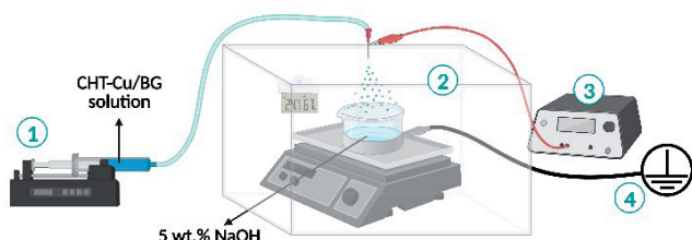
Fig. 1. Schematic illustration of electro spraying setup. 1 - syringe pump; 2 - isolating chamber; 3 - high voltage generator; 4 - grounding. Created with BioRender.com.
