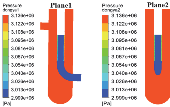
Figure 8 Pressure cloud images of plane 1 and plane 2
