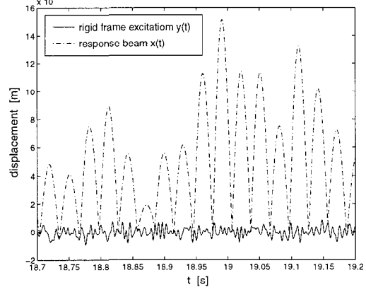
Figure 8: Parts of time series: 200 Hz band excitation y(t) and response beam x(t)
