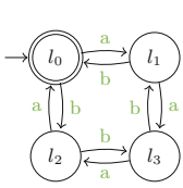
(a) A DFA \mathcal{A}
