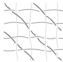
Untwisted weave in \mathbb{X}^3 = \mathbb{E}^2 \times I , with I = [-1, 1] .
